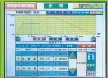
■ 溶接条件設定画面(任意波形) Setting of welding condition display view
