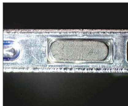
携帯2次電池 封止溶接 Seal welding for rechargeable battery
