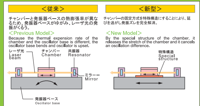
■ 高安定構造 Figure of High-Stability Structure
